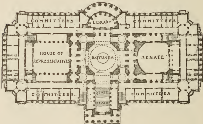
MISSOURI STATE CAPITOL, JEFFERSON CITY, MO. .
